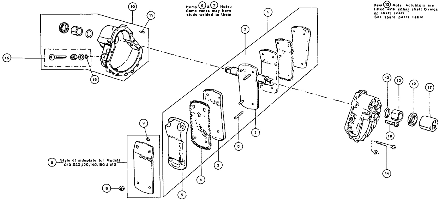
EXPLODED VIEW OF A TYPICAL STANDARD ACTUATOR
