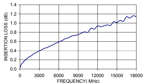
086-12SM+ INSERTION LOSS
